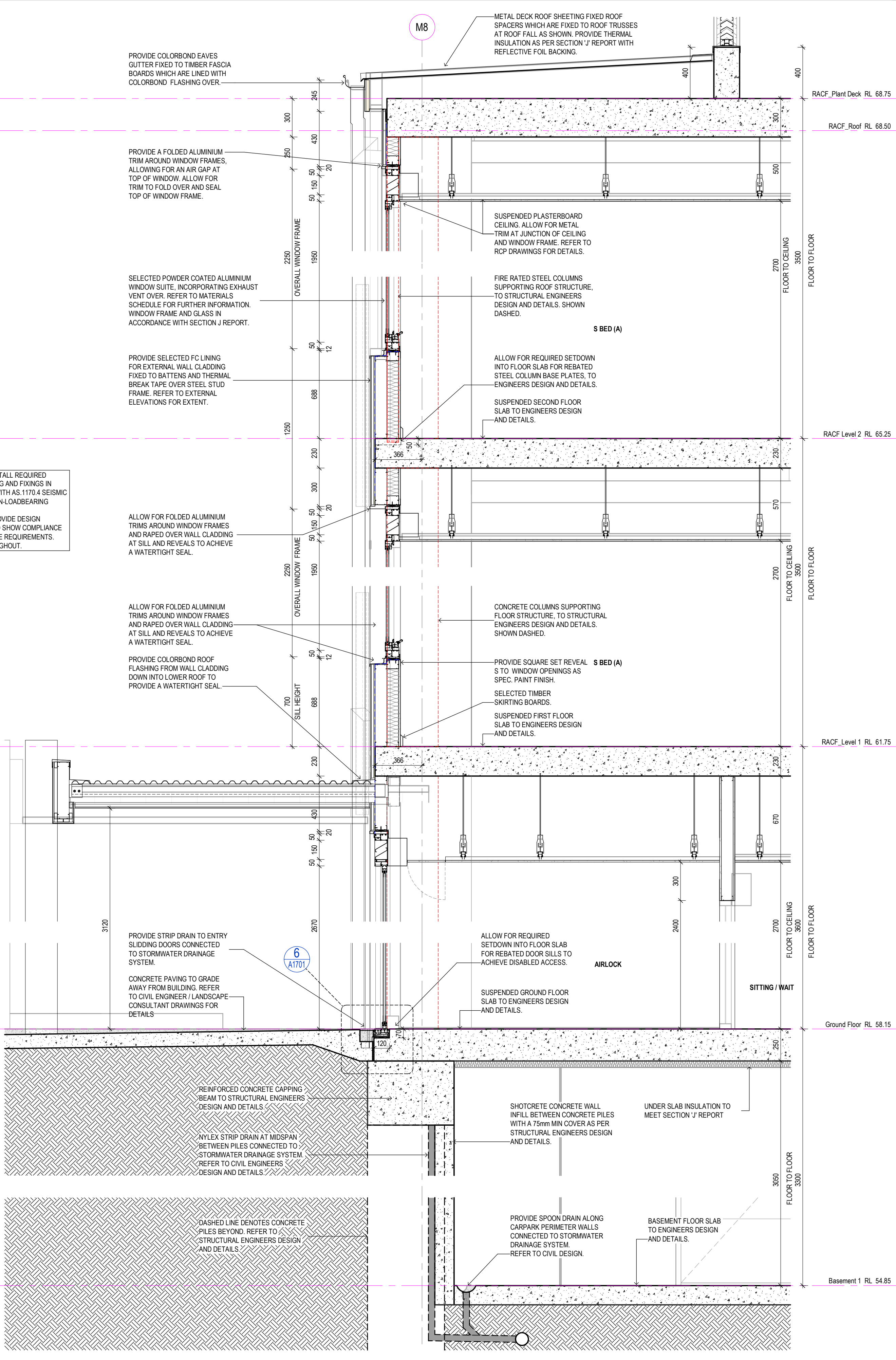
3 RACF - WALL SECTION 03 Scale 1:20
